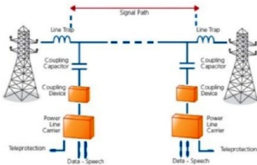
Phase-to-ground coupling
